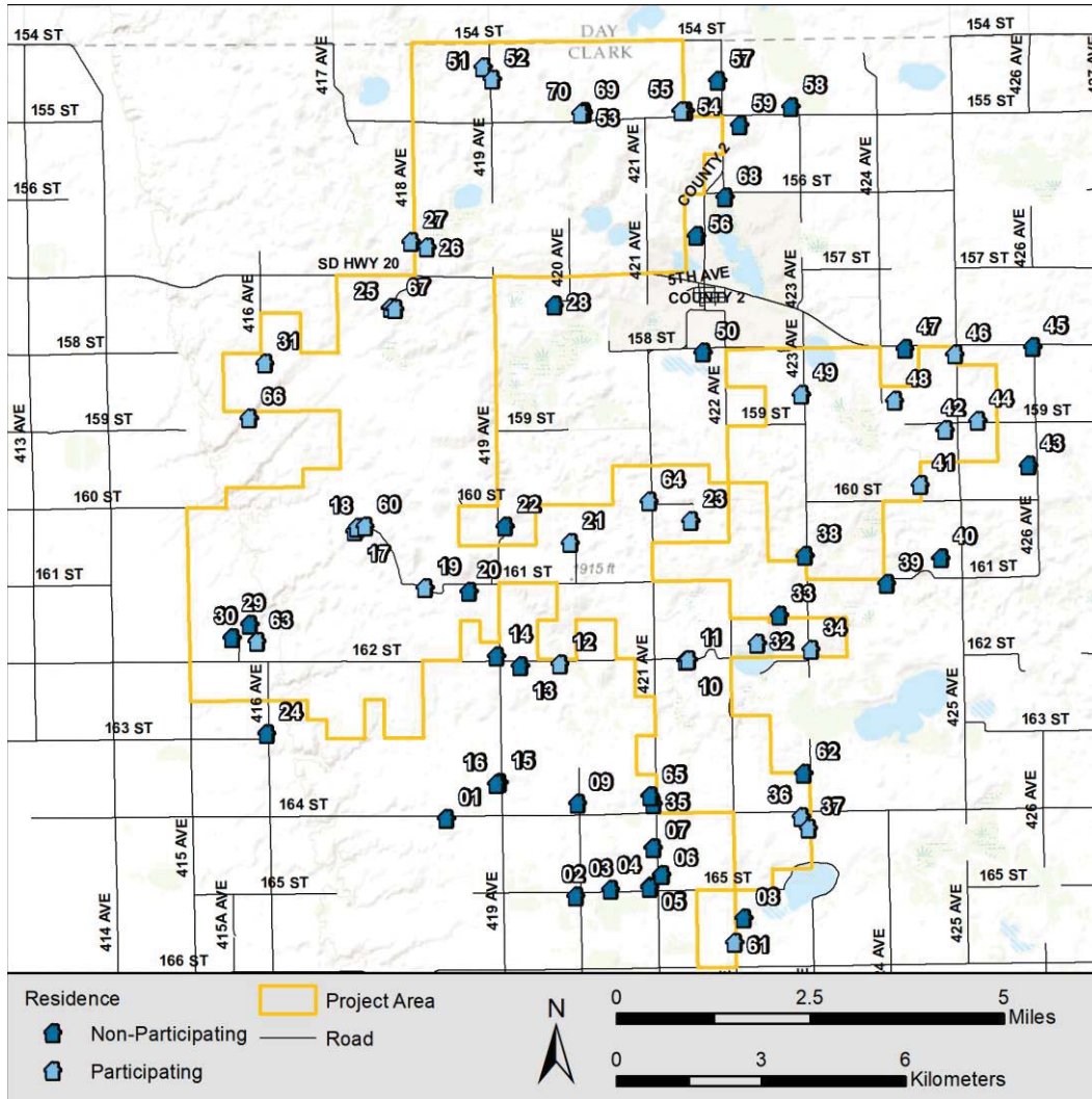
FIGURE 25: RECEIVER LOCATIONS AND SOUND PROPAGATION MODELING RESULTS
