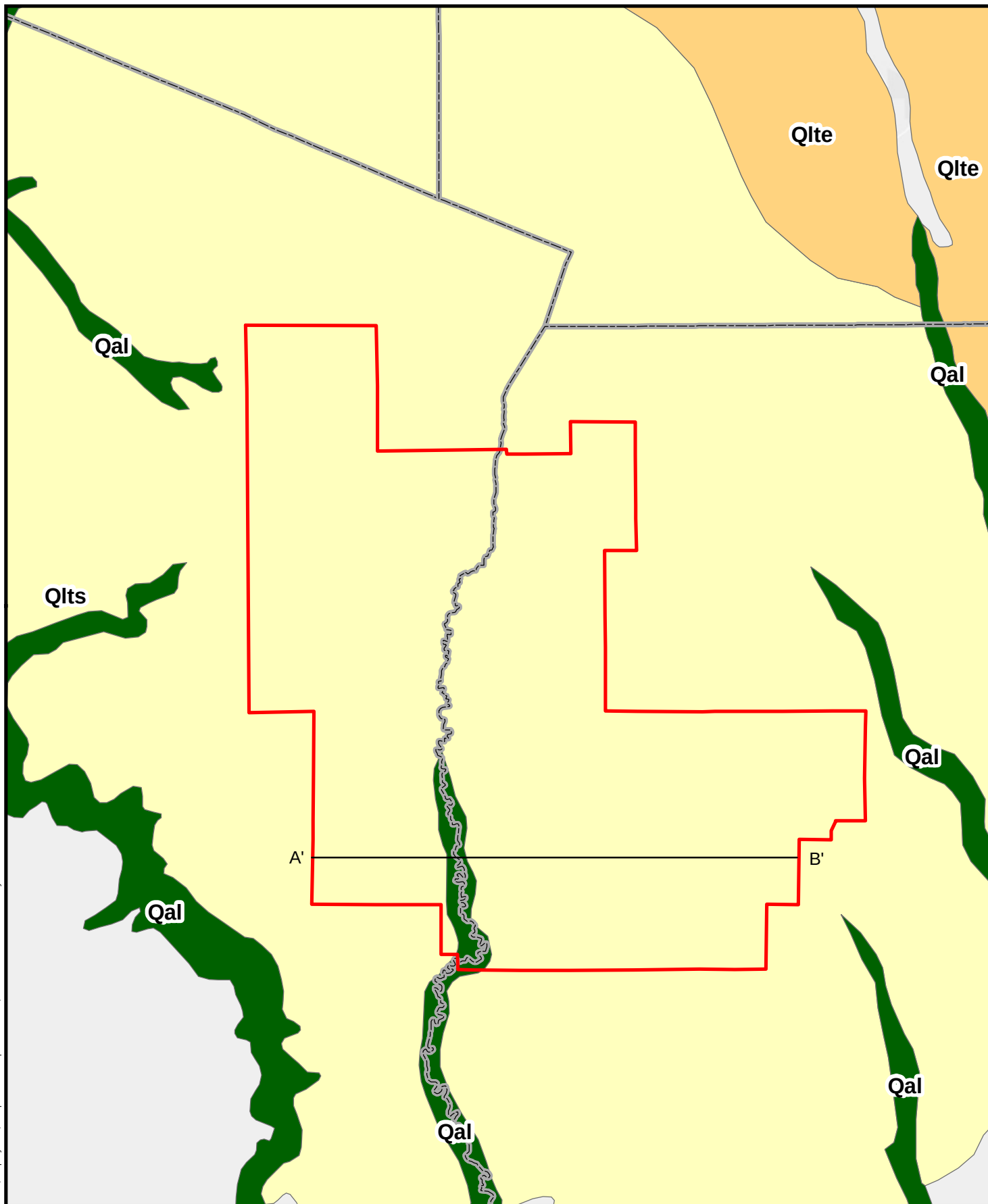
Figure 6a Surficial Geology Prevailing Winds, LLC Wind Energy Facility SDPUC Application
