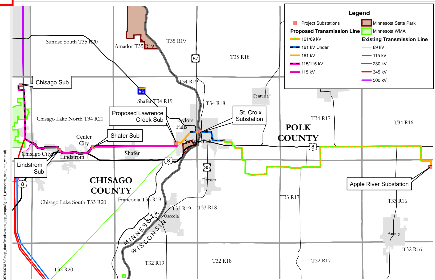
Figure 1 - Project Overview Map Chisago County to Apple River 115 kV/161 kV Transmission Line Project Xcel Energy Chisago County, Minnesota
