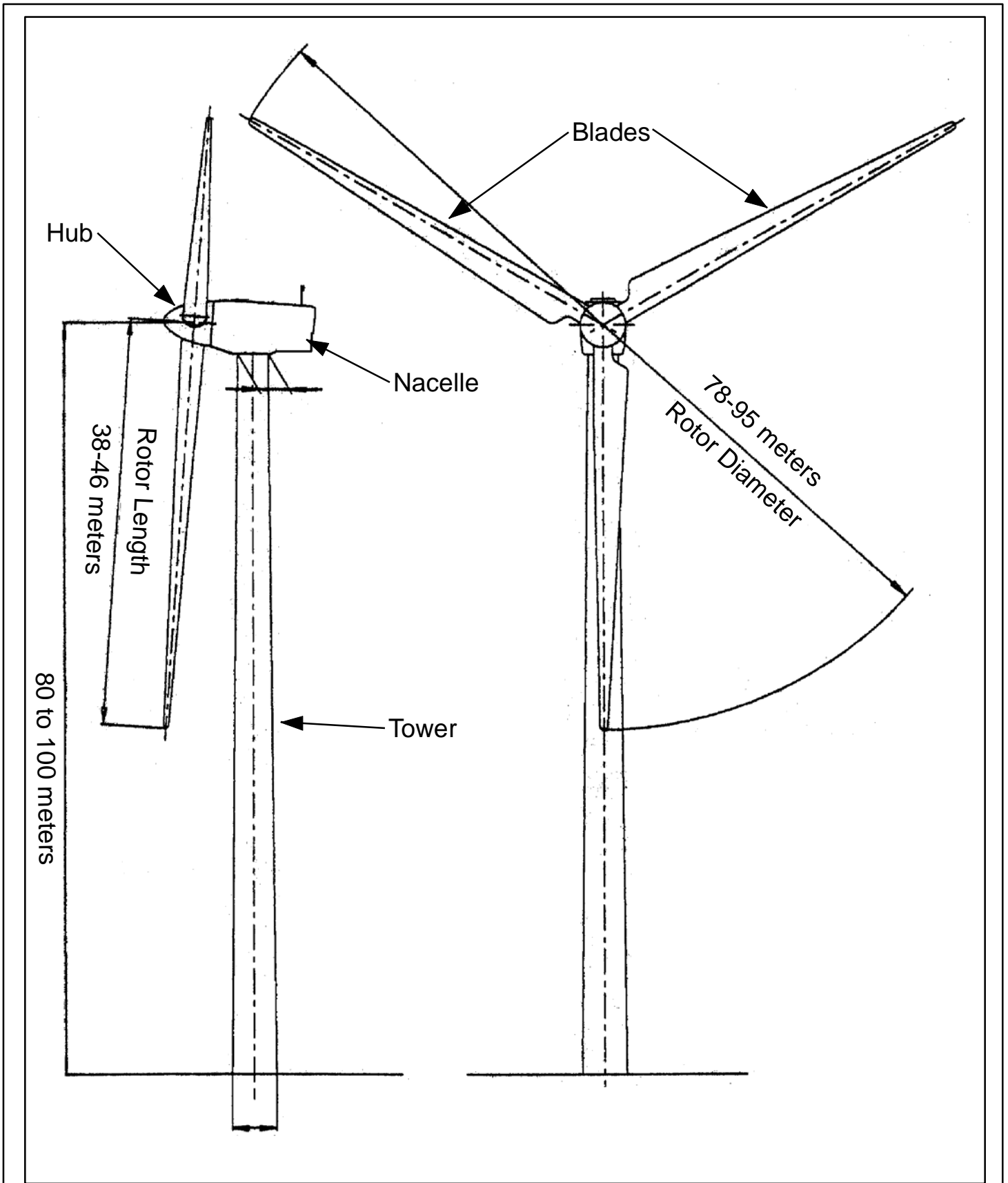
Figure 4 - Wind Turbine Generator Typical Dimensions Buffalo Ridge II Wind Farm Iberdrola Renewables Brookings and Deuel Counties, SD
