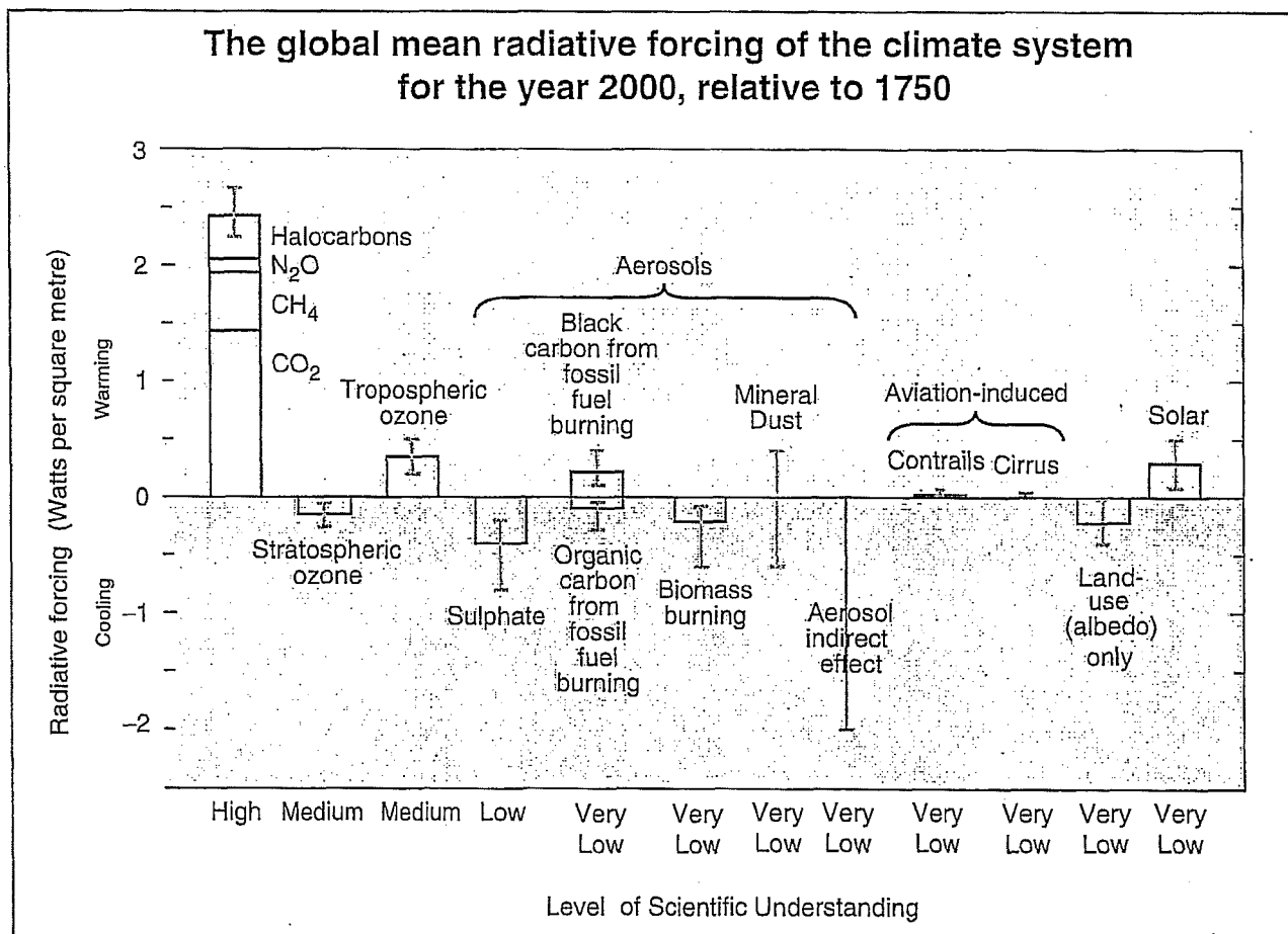
Figure 3: Many external factors force climate change.
