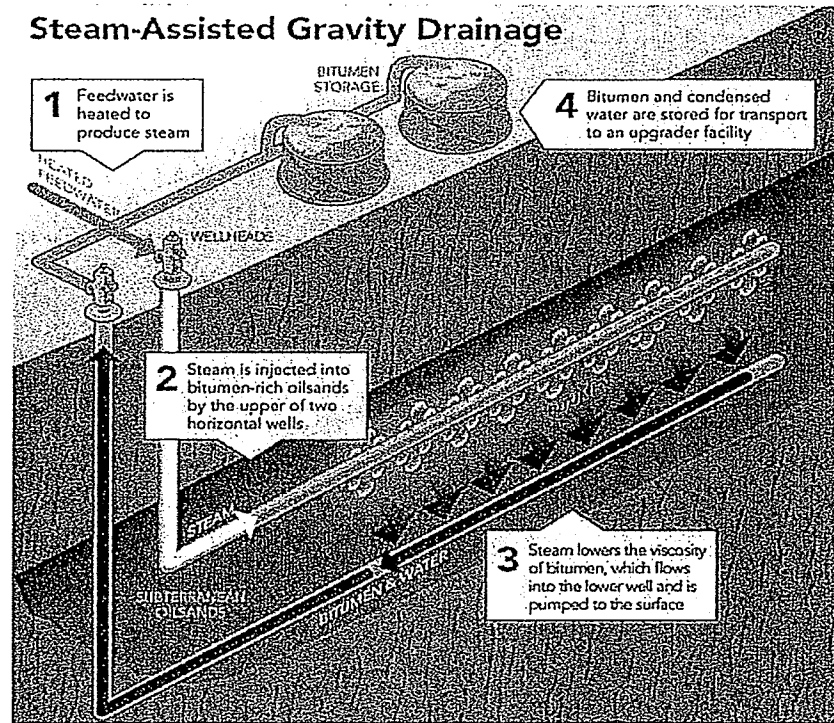
FIGURE 3-3 Bitumen recovered using SAGD (ERCB 2012b).
