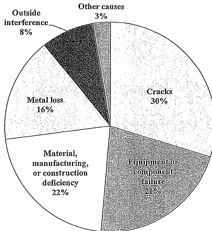
FIGURE 4-4 Causes of crude oil transmission pipeline incidents reported to NEB, 2004 to 2011. (Source: TSB 2012, Table 5.)
