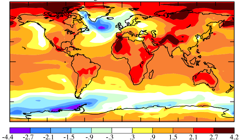
2055-2060 Surface Air Temperature (°C) Relative to 1880-1920 A1B + Modified Forcings, Ice Melt to 1 m 1.19
