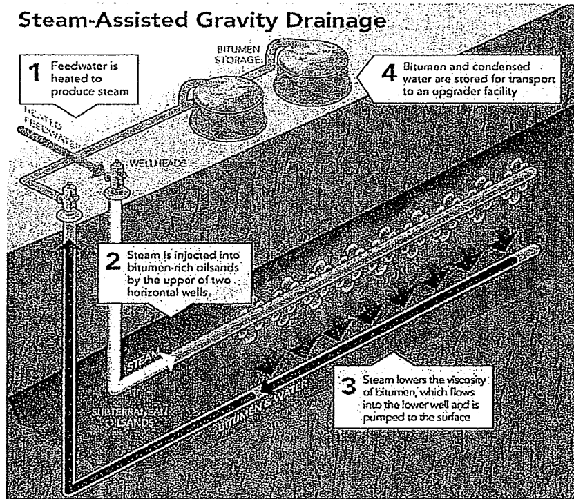
FIGURE 3-3 Bitumen recovered using SAGD (ERCB 2012b).
