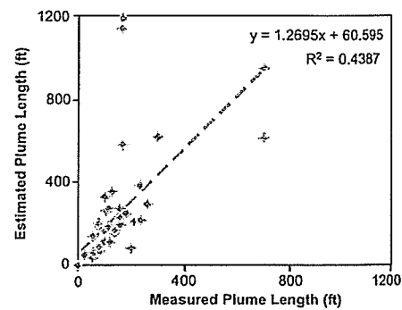
Fig. 1. Correlation between estimated and measured plume lengths at 30 UST sites with well-delineated MTBE, benzene, and TBA plumes
